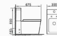
BR-T004B Washdown two-piece toilet Size: 675×355×830mm S-trap, 250mm Roughing-in P-trap, 180mm Roughing-in
