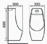
BR-71 Wall-hung Urinal Size: 350×300×690mm
