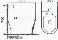
BR-0313 Excess eddy one-piece toilet Size: 660×350×700mm S-trap,220/250/300mm Roughing-in
