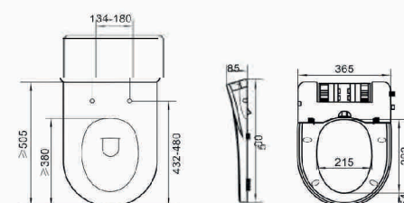
BS002 Bidet Seat Size: 500×365×85mm
