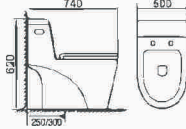
BR-0319 Siphonic one-piece toilet Size: 740×500×620mm S-trap,250/300mm Roughing-in
