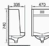
BR-73 Wall-hung Urinal Size: 470×335×740mm
