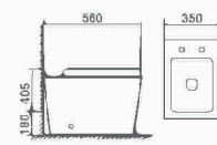
BR-HT9017B Back to wall toilet Size: 560×350×405mm P-trap, 180mm Roughing-in
