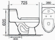
BR-0335B Siphonic one-piece toilet Size: 725×380×635mm S-trap,300mm Roughing-in
