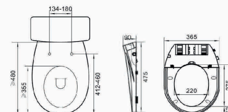
BS001 Bidet Seat Size: 475×365×90mm
