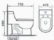
BR-0334 Siphonic one-piece toilet Size: 710×410×590mm S-trap,250/300mm Roughing-in
