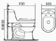
BR-0335A Siphonic one-piece toilet Size: 700×350×630mm S-trap,250/300mm Roughing-in
