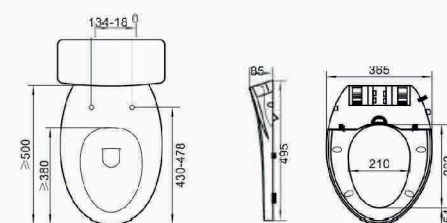
BS003 Bidet Seat Size: 495×365×85mm
