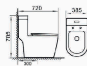
Sofitel Siphonic one-piece toilet Size: 720×385×705mm S-trap, 300mm Roughing-in
