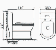
BR-0322 Excess eddy one-piece toilet Size: 710×380×770mm S-trap,250/300mm Roughing-in
