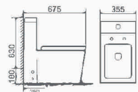
BR-T004B Washdown two-piece toilet Size: 675×355×830mm S-trap, 250mm Roughing-in P-trap, 180mm Roughing-in
