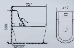
Lima Intelligent toilet Size: 721x417x580mm S-trap, 300/400mm Roughing-in
