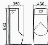
BR-70 Stand-hung Urinal Size: 430×350×980mm
