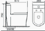
BR-0312 Washdown one-piece toilet Size: 670×360×750mm S-trap,250/300mm Roughing-in
