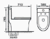
Feri Eddy double hole one-piece closet Size: 710×385×745mm S-trap, 220/250/300/400mm Roughing-in
