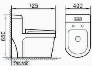
BR-0330 Excess eddy one-piece toilet Size: 725×400×650mm S-trap,250/300mm Roughing-in
