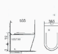
BR-HT9034B Back to wall toilet Size: 565×365×410mm S-trap, 120/150mm Roughing-in P-trap, 180mm Roughing-in
