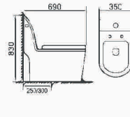
BR-0342 Excess eddy one-piece toilet Size: 690×350×830mm S-trap,250/300mm Roughing-in
