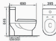
BR-0346 Washdown one-piece toilet Size: 690×395×645mm S-trap,250/300mm Roughing-in
