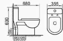
BR-0348 Washdown one-piece toilet Size: 680×355×690mm S-trap,250/300mm Roughing-in P-trap,180mm Roughing-in
