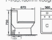
Cochin Siphonic one-piece toilet Size: 670×360×730mm S-trap, 220/300mm Roughing-in Washdown one-piece toilet S-trap, 100mm Roughing-in P-trap, 180mm Roughing-in
