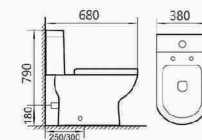
BR-9014A Washdown two-piece Toilet Size: 680×380×790mm S-trap, 250/300mm Roughing-in P-trap, 180mm Roughing-in
