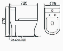
BR-0344 4DExcess eddy one-piece toilet Size: 720×425×770mm S-trap,200/250/300mm Roughing-in
