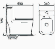
BR-0328 Siphonic one-piece toilet Size: 680×360×755mm S-trap,250/300mm Roughing-in
