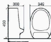
BR-75 Wall-hung Urinal Size: 340×300×490mm
