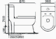
BR-0337 Washdown one-piece toilet Size: 670×360×700mm S-trap,200/250/300mm Roughing-in P-trap,180mm Roughing-in
