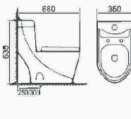
BR-0321 Washdown one-piece toilet Size: 680×350×635mm S-trap,250/300mm Roughing-in
