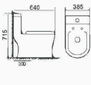
BR-0340 Excess eddy one-piece toilet Size: 640×385×715mm S-trap,300mm Roughing-in
