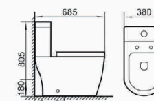
BR-T003B Washdown two-piece toilet Size: 685×380×805mm S-trap, 250mm Roughing-in P-trap, 180mm Roughing-in
