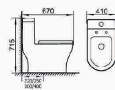
Oscar Eddy double hole one-piece closet Size: 670×410×715mm S-trap, 220/250/300/400mm Roughing-in
