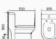
BR-0336 Washdown one-piece closet Size: 700×370×800mm S-trap,100/200/250mm Roughing-in P-trap,180mm Roughing-in
