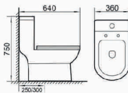
BR-0345 Excess eddy one-piece toilet Size: 640×360×750mm S-trap,250/300mm Roughing-in
