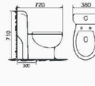
BR-0341 Siphonic one-piece toilet Size: 720×380×710mm S-trap,300mm Roughing-in
