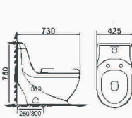
BR-0320 Washdown one-piece toilet Size: 730×425×750mm S-trap,250/300mm Roughing-in
