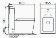
BR-T004 Washdown Siphonic one-piece toilet Size: 670×355×810mm Siphonic: S-trap, 250/300mm Roughing-in Washdown: S-trap, 250mm Roughing-in P-trap, 180mm Roughing-in
