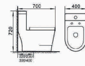
Lyon Eddy double hole one-piece closet Size: 700×400×720mm S-trap, 220/250/300/400mm Roughing-in
