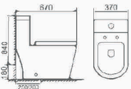
BR-T003 Washdown Siphonic one-piece toilet Size: 670×370×840mm Siphonic: S-trap, 300mm Roughing-in Washdown: S-trap, 250mm Roughing-in P-trap, 180mm Roughing-in
