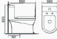
BR-0338 Excess eddy one-piece toilet Size: 660×360×695mm S-trap,300mm Roughing-in
