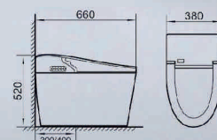
Beira Intelligent toilet Size: 660x380x520mm S-trap, 300/400mm Roughing-in
