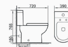
BR-9014A Washdown two-piece Toilet Size: 720×390×765mm S-trap, 250/300mm Roughing-in P-trap, 180mm Roughing-in
