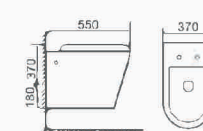
BR-HT9034 Wall-hung toilet Size: 550×370×370mm P-trap, 180mm Roughing-in
