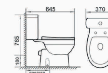
BR-9100A Washdown two-piece Toilet Size: 645×370×765mm S-trap, 200/250mm Roughing-in P-trap, 180mm Roughing-in
