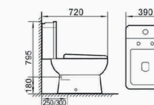
BR-9104 Washdown two-piece Toilet Size: 720×390×795mm S-trap, 250/300mm Roughing-in P-trap, 180mm Roughing-in
