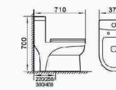
kimberly Collision type flush one-piece toilet Size: 710×370×700mm S-trap, 220/250/300/400mm Roughing-in
