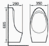
BR-72 Wall-hung Urinal Size: 350×290×685mm
