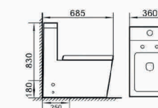
BR-T001B Washdown two-piece toilet Size: 685×360×830mm S-trap, 250mm Roughing-in P-trap, 180mm Roughing-in
